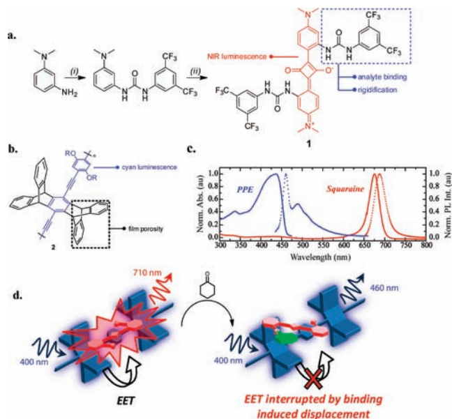
Figure 1. (a) Synthesis of squaraine reporter dye 1 . (i) 3,5-Bis(trifluoromethyl)phenyl isocyanate, CH 2 Cl 2 , rt, 12 h. (ii) Squaric acid, toluene/ n -butanol (3:1), reflux, 6 h. (b) Molecular structure of PPE 2 (R = C 14 H 29 ). (c) Absorbance (solid line) and photoluminescence (circles) spectra of PPE 2 (blue) and squaraine 1 (red). PPE 2 photoluminescence spectra are from a thin film; all other measurements taken in CHCl 3 ( 2 λ ex = 380 nm, 1 λ ex = 660 nm). The red shift of the emission maximum of 1 in thin films is likely due to stabilization of the excited state of 1 in the polymer matrix.
